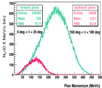
(a). 500 MeV incident protons.
