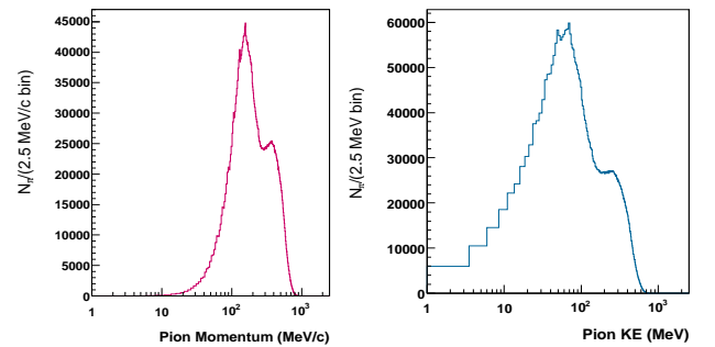
(b) 1 GeV
