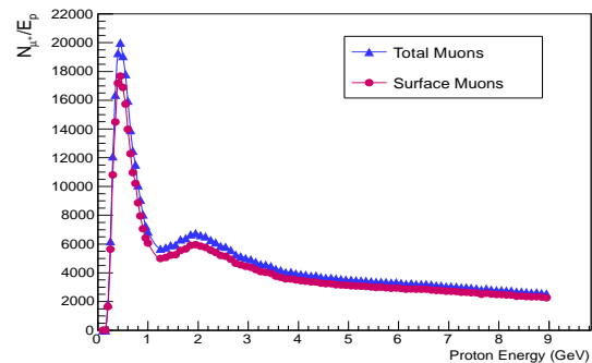
(b). Yield normalised to proton energy.
