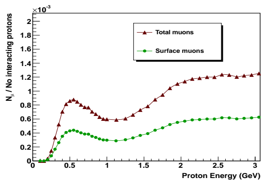
(c). Muon yield normalised to the number of protons interacting in the target.
