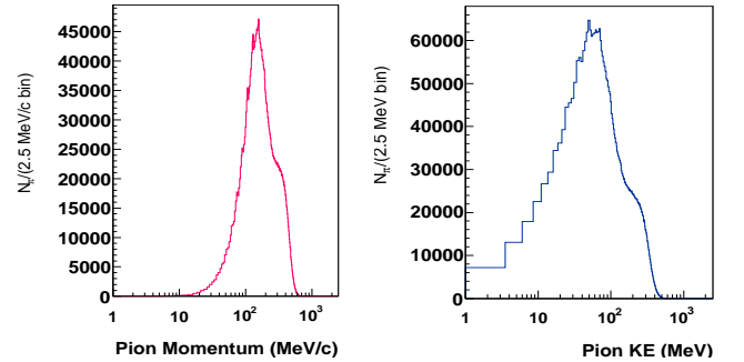
(a) 750 MeV
