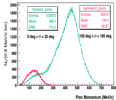
(b). 800 MeV incident protons.
